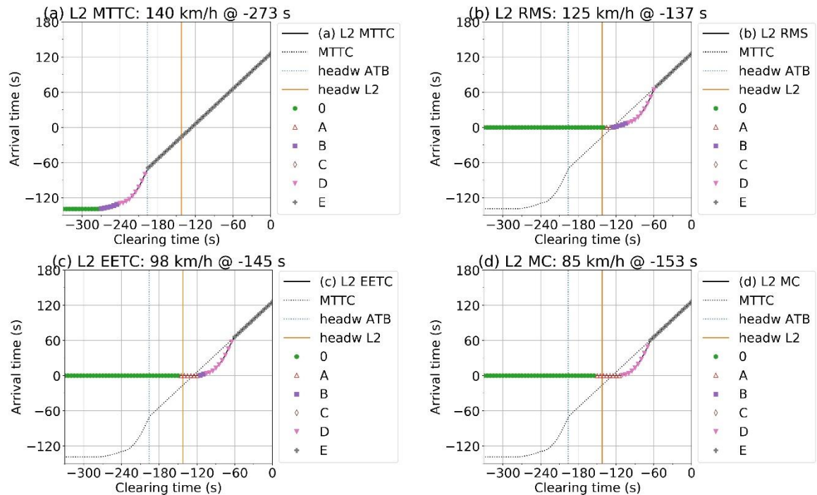
Figure 5: Arrival times under ETCS L2 (a) MTTC, (b) RMS, (c) EETC, (d) MC. . Markers show the obstruction classes (L2 0 to L2 E, see Figure 3); headw ATB= headway shows the NS'54/ATB headway as a reference; headw L2 = headway ETCS L2..
